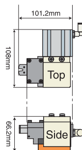
TKC-B1 (external dimension diagram)
