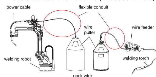
Flexible Conduit Use Positions (Robot/Semi-Auto)
