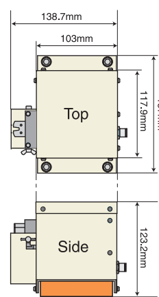
TKC-A2 (external dimension diagram)
